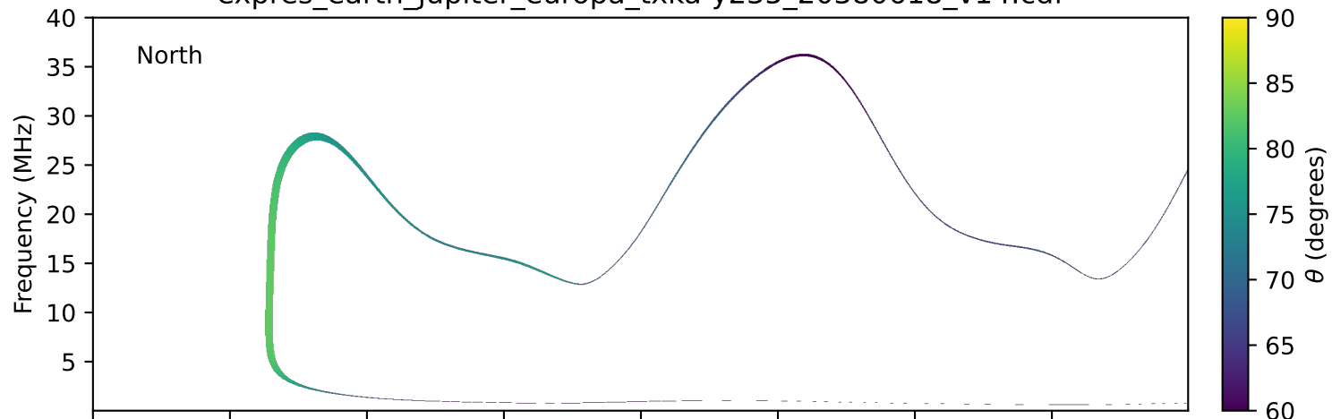
expres_earth_jupiter_europa_txka-y235_20380618_v14.cdf
