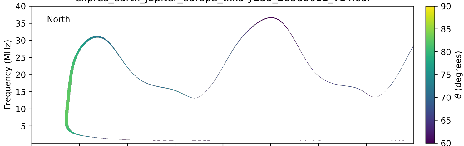
expres_earth_jupiter_europa_txka-y235_20380611_v14.cdf
