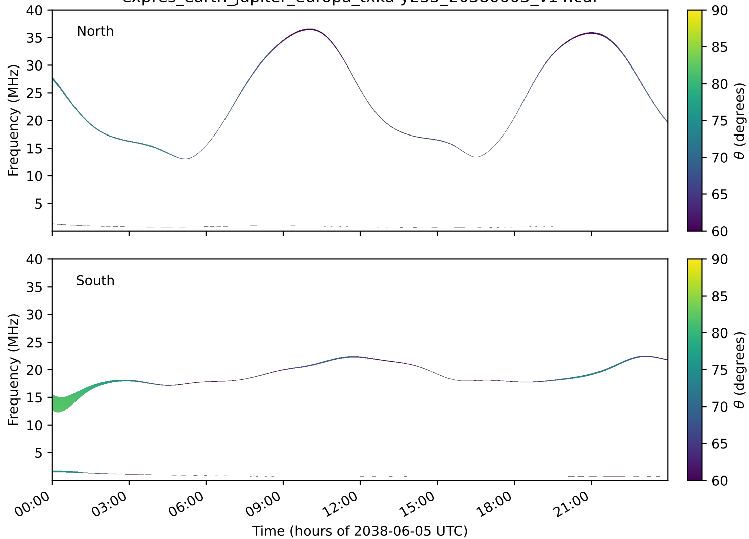
expres_earth_jupiter_europa_txka-y235_20380605_v14.cdf
