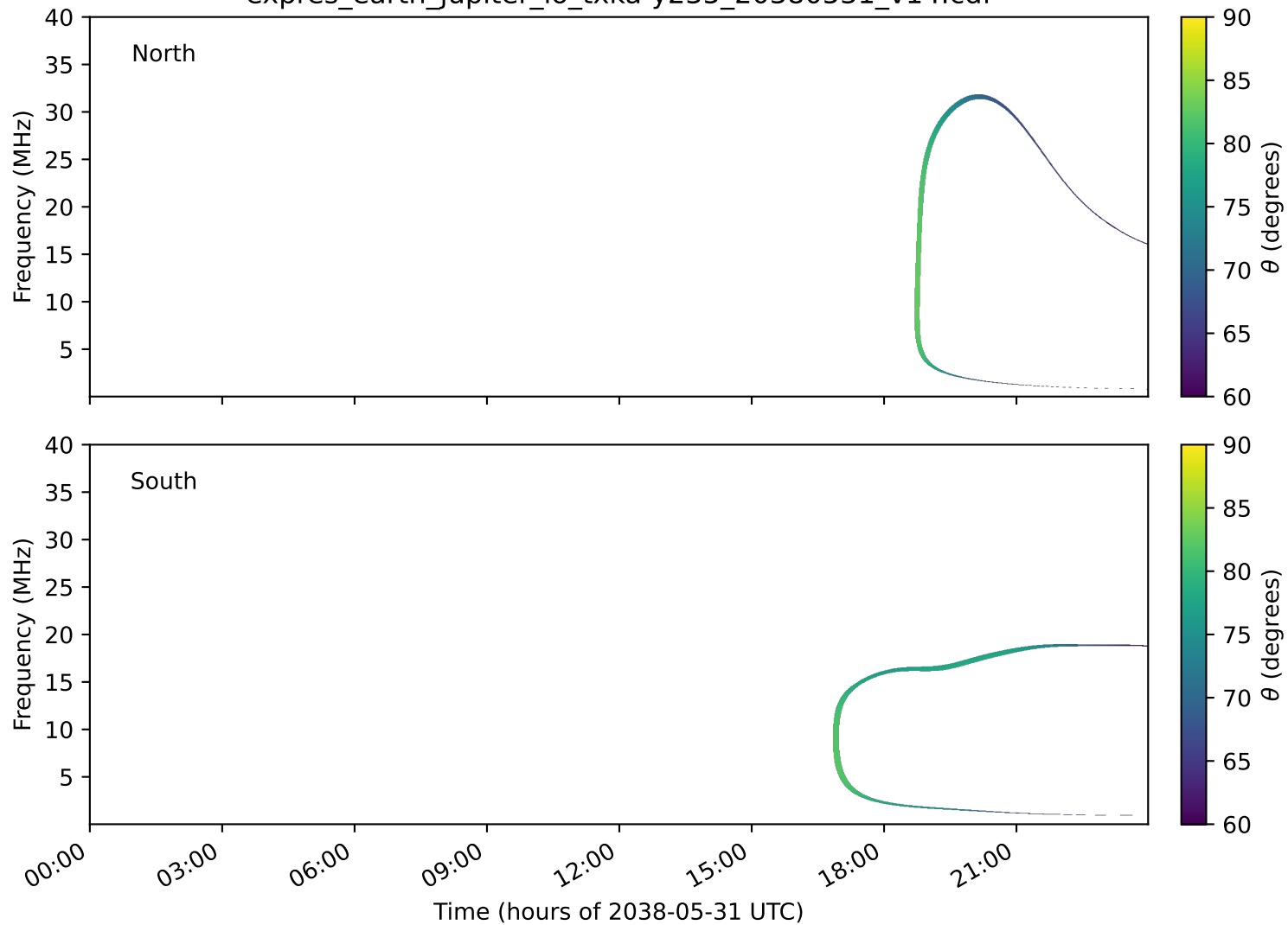
expres_earth_jupiter_io_txka-y235_20380531_v14.cdf
