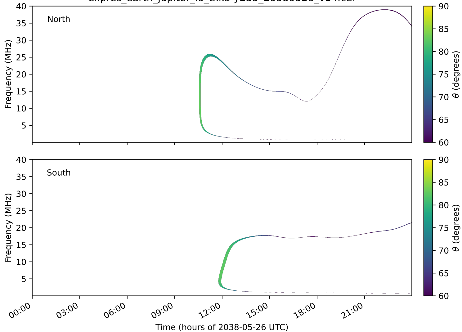
expres_earth_jupiter_io_txka-y235_20380526_v14.cdf
