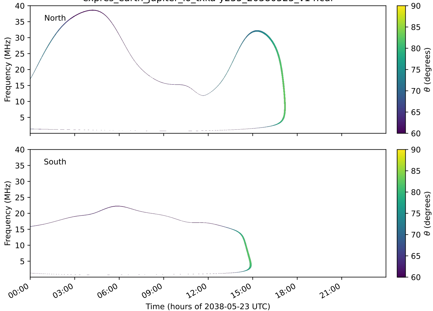
expres_earth_jupiter_io_txka-y235_20380523_v14.cdf
