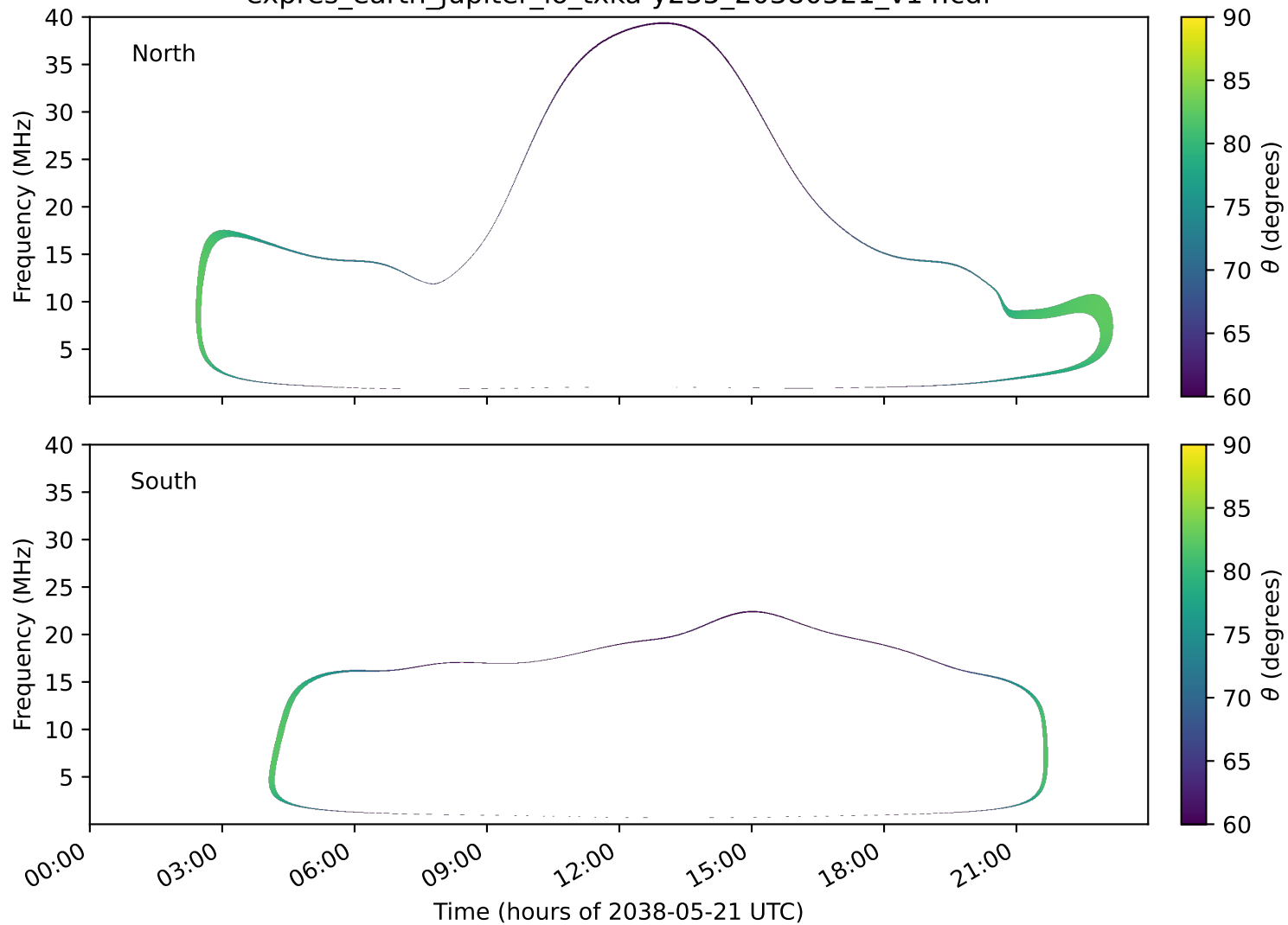
expres_earth_jupiter_io_txka-y235_20380521_v14.cdf
