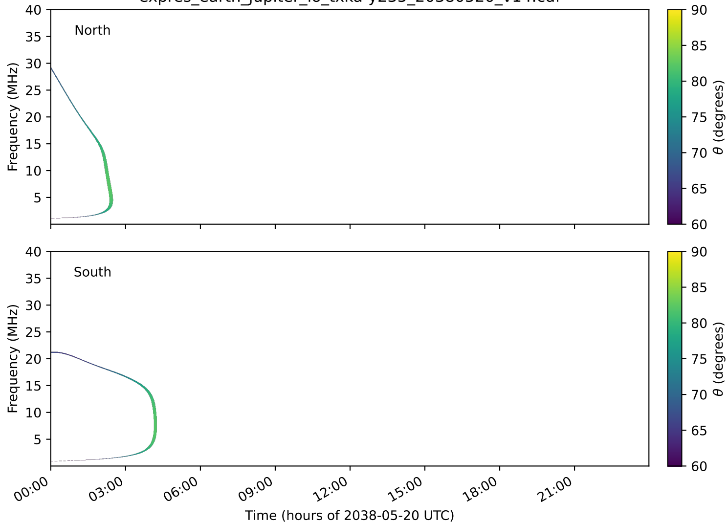
expres_earth_jupiter_io_txka-y235_20380520_v14.cdf
