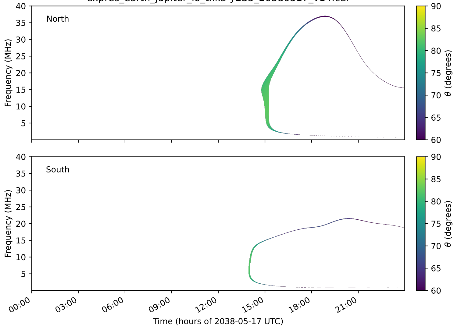
expres_earth_jupiter_io_txka-y235_20380517_v14.cdf
