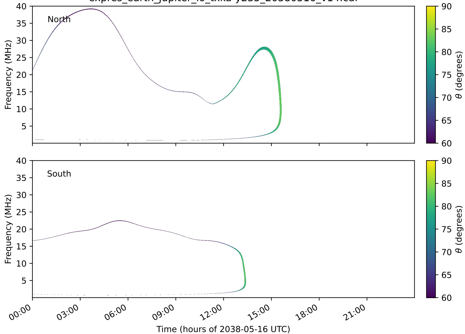
expres_earth_jupiter_io_txka-y235_20380516_v14.cdf
