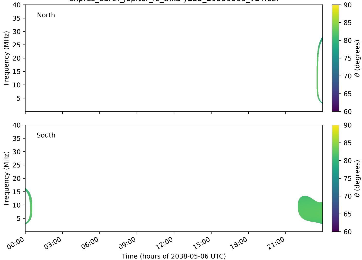
expres_earth_jupiter_io_txka-y235_20380506_v14.cdf
