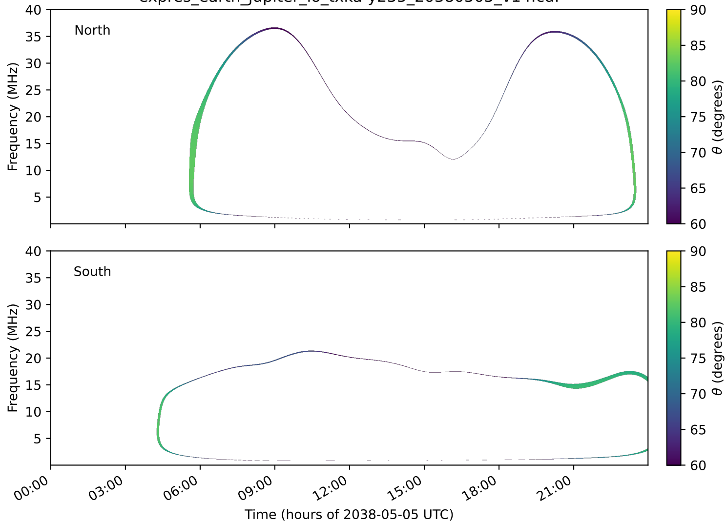
expres_earth_jupiter_io_txka-y235_20380505_v14.cdf
