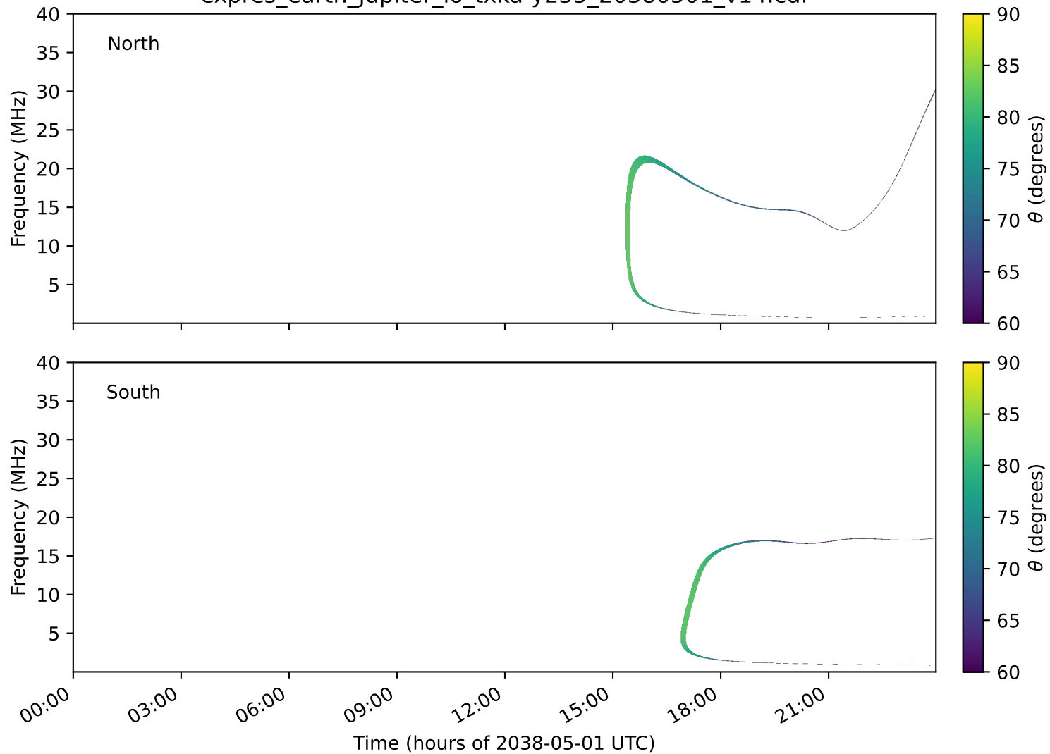
expres_earth_jupiter_io_txka-y235_20380501_v14.cdf
