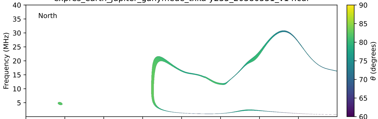
expres_earth_jupiter_ganymede_txka-y235_20380531_v14.cdf
