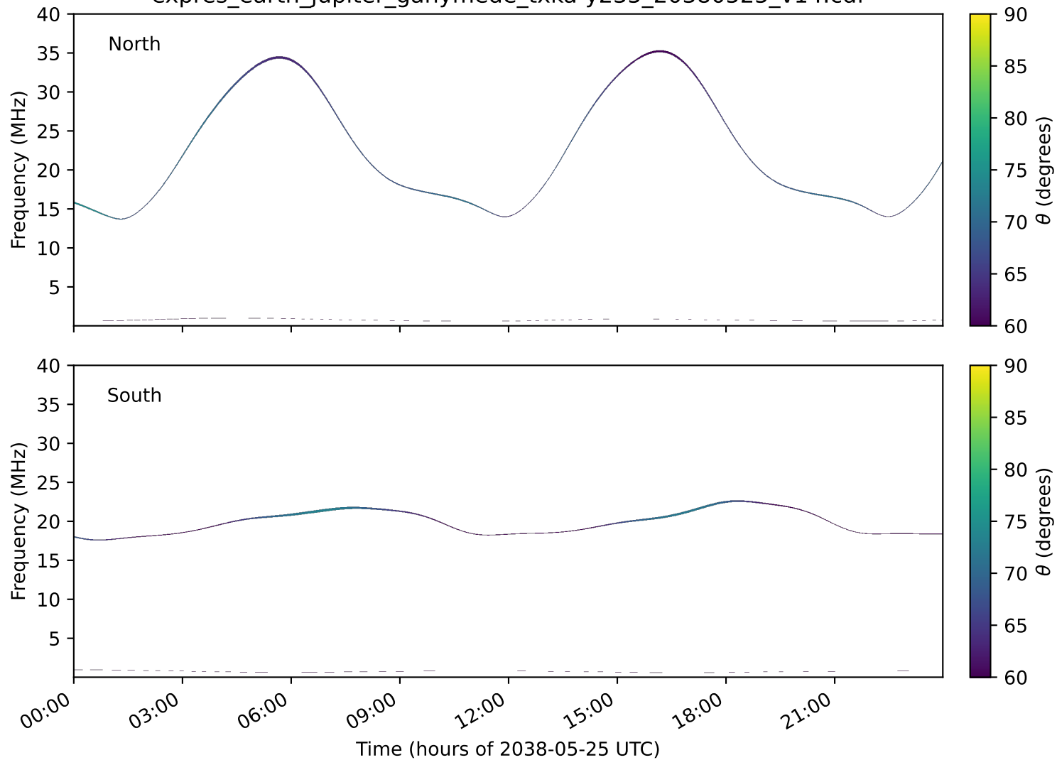
expres_earth_jupiter_ganymede_txka-y235_20380525_v14.cdf
