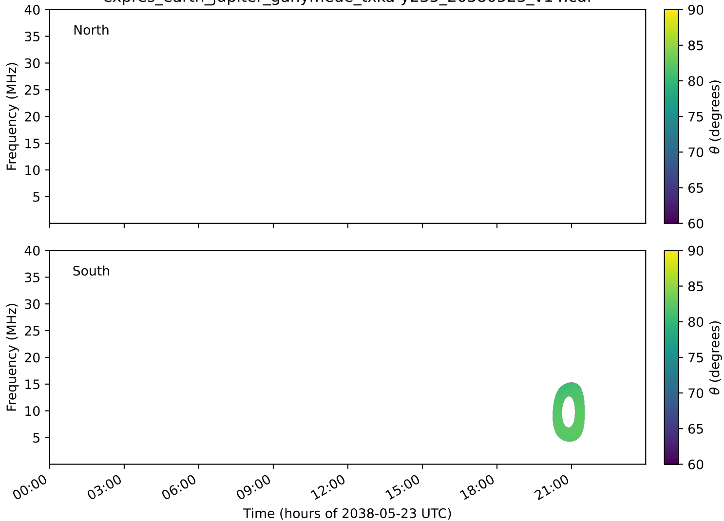
expres_earth_jupiter_ganymede_txka-y235_20380523_v14.cdf
