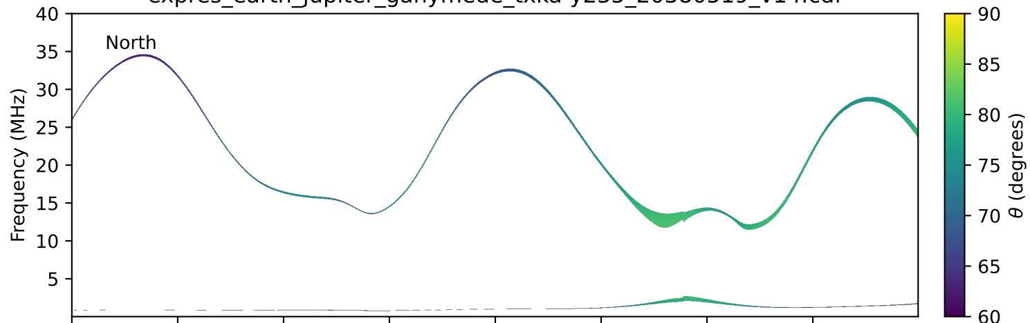
expres_earth_jupiter_ganymede_txka-y235_20380519_v14.cdf
