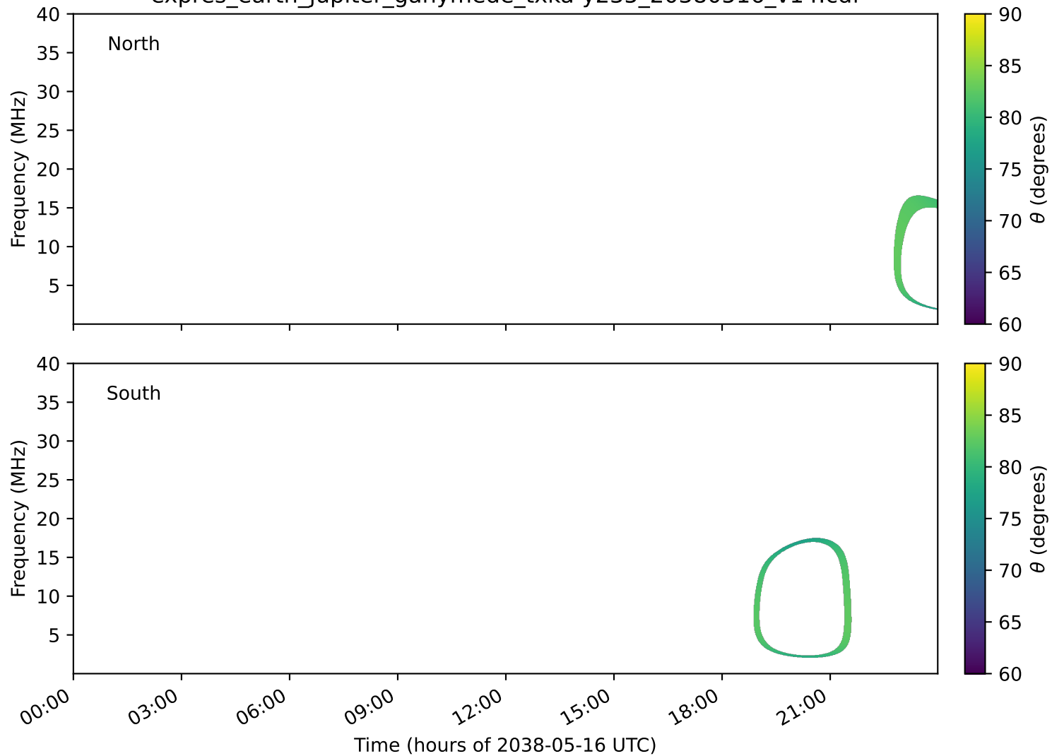
expres_earth_jupiter_ganymede_txka-y235_20380516_v14.cdf
