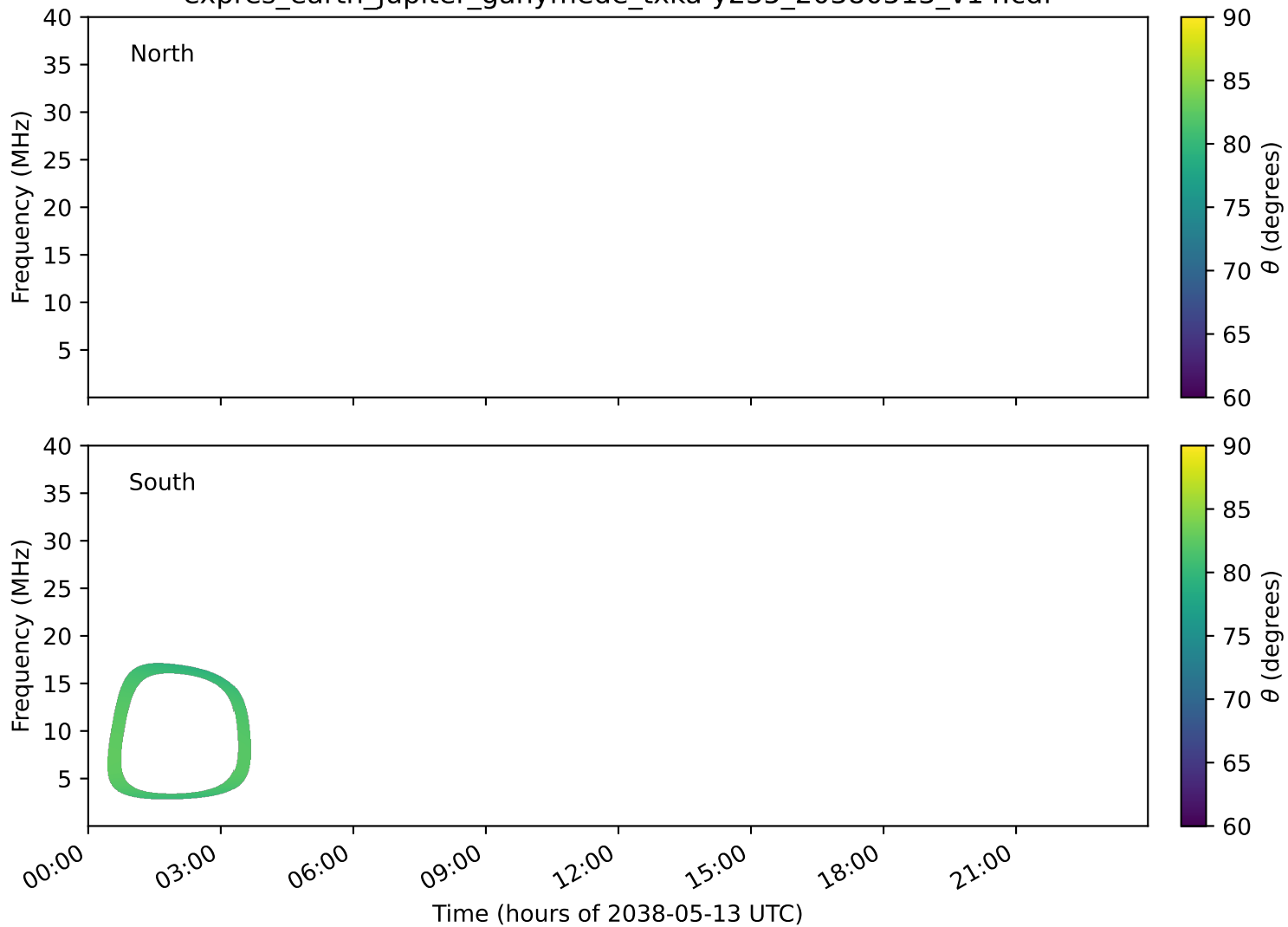
expres_earth_jupiter_ganymede_txka-y235_20380513_v14.cdf
