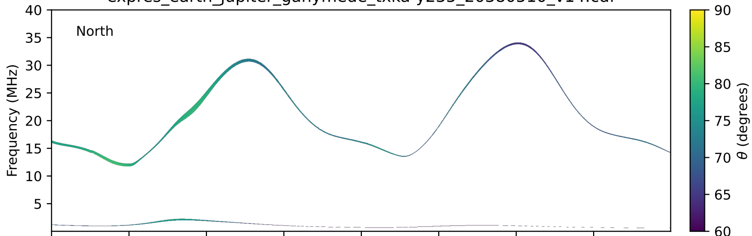
expres_earth_jupiter_ganymede_txka-y235_20380510_v14.cdf
