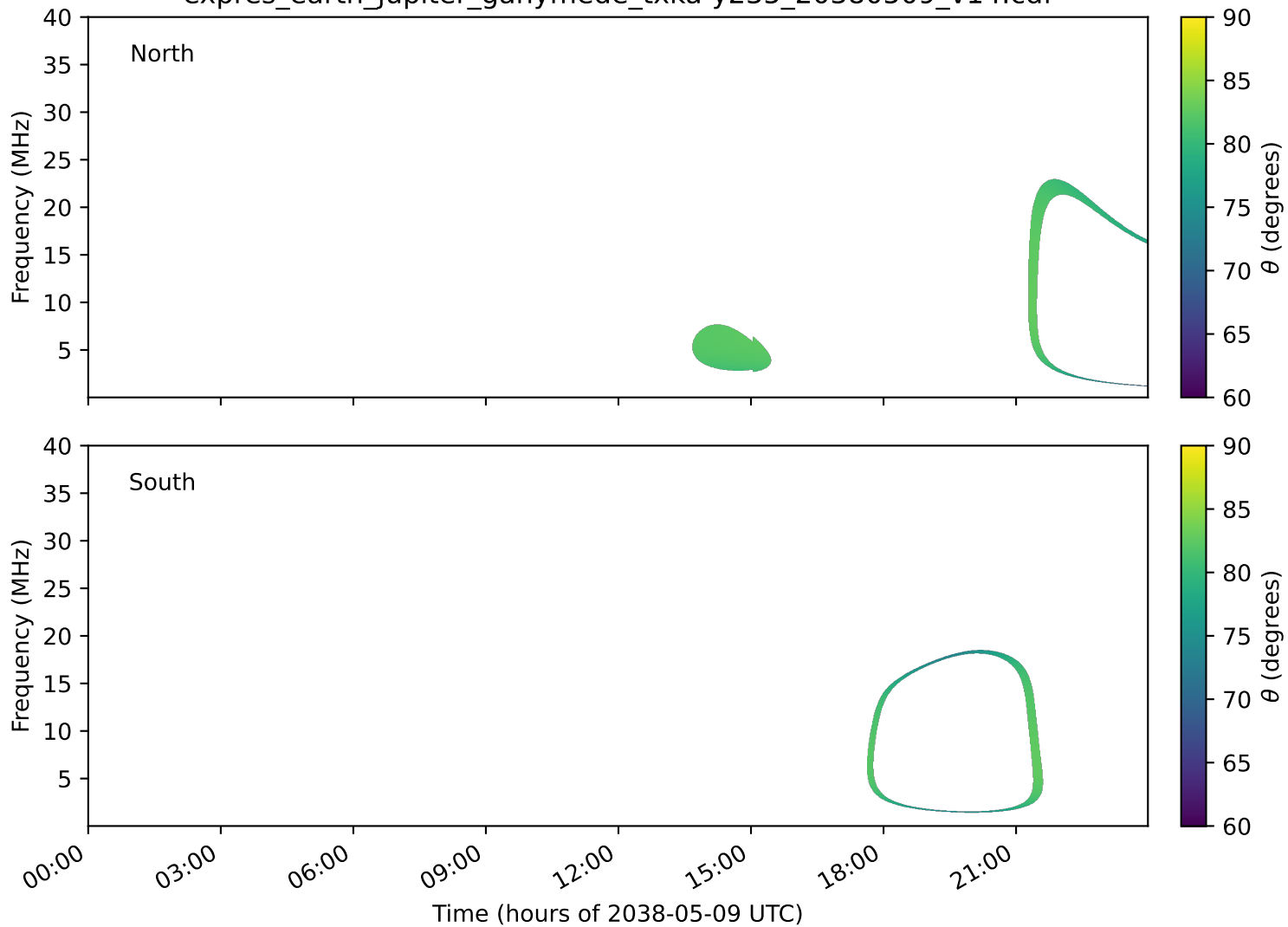
expres_earth_jupiter_ganymede_txka-y235_20380509_v14.cdf
