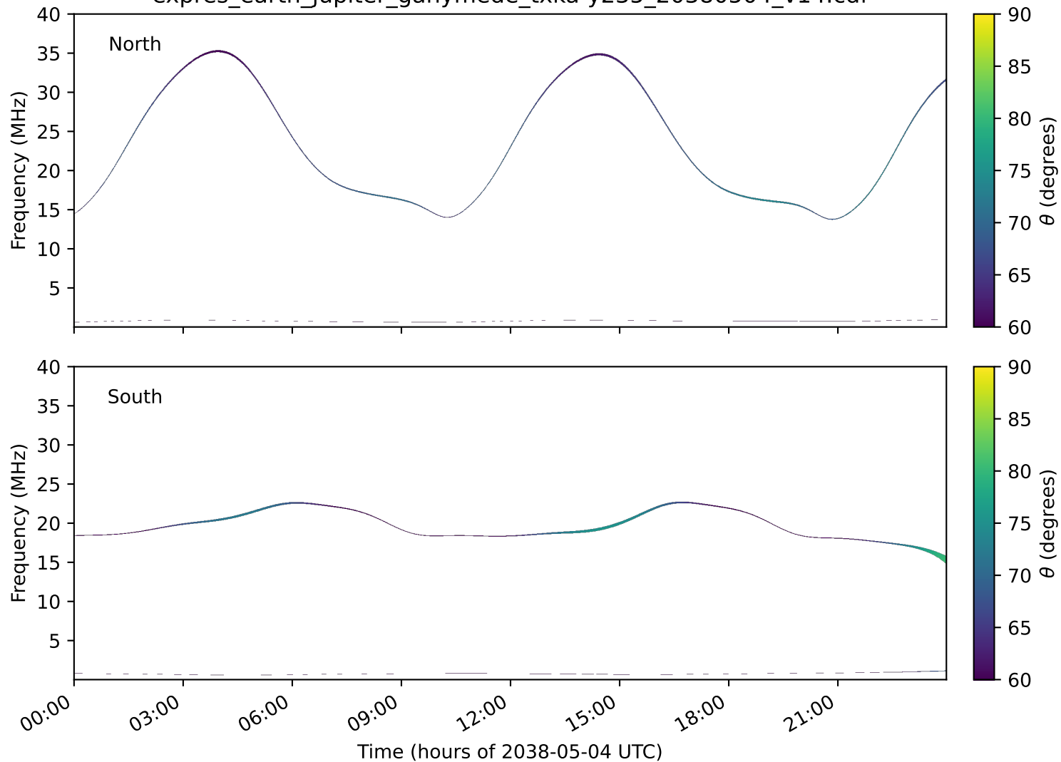
expres_earth_jupiter_ganymede_txka-y235_20380504_v14.cdf
