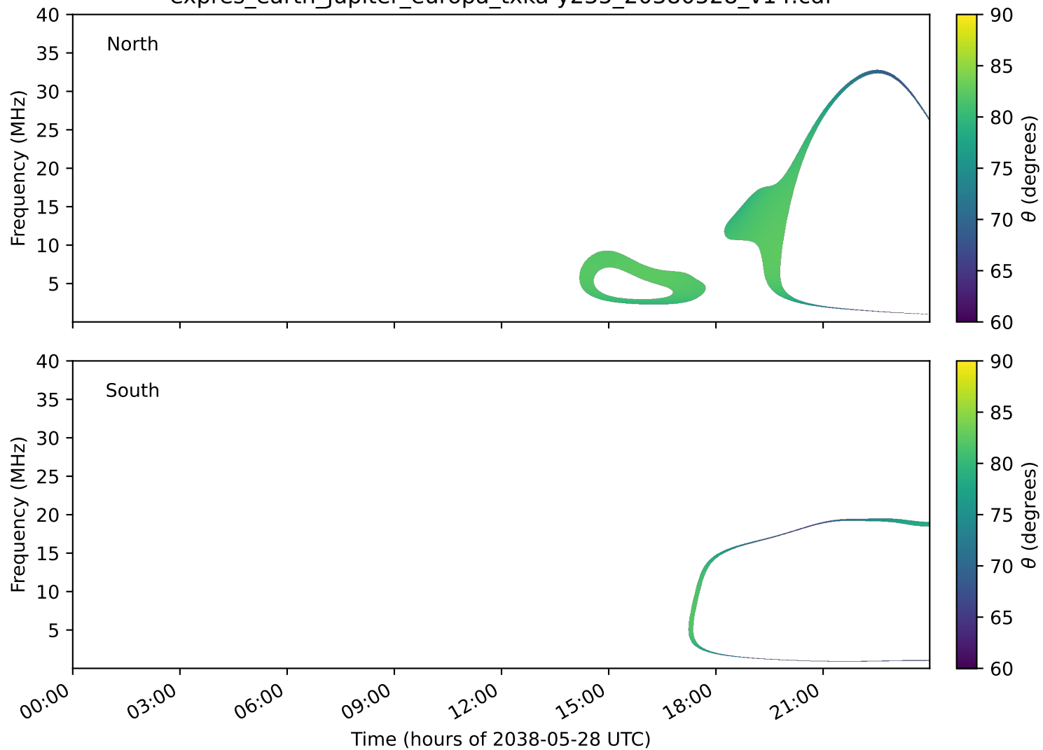
expres_earth_jupiter_europa_txka-y235_20380528_v14.cdf
