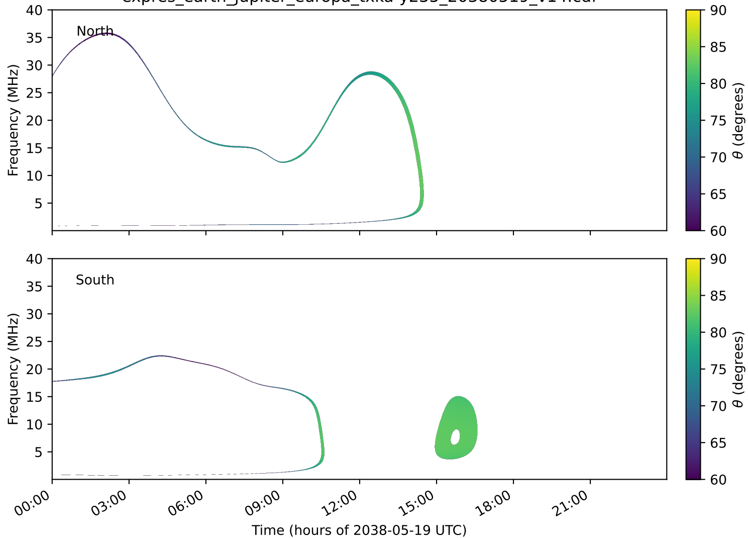
expres_earth_jupiter_europa_txka-y235_20380519_v14.cdf
