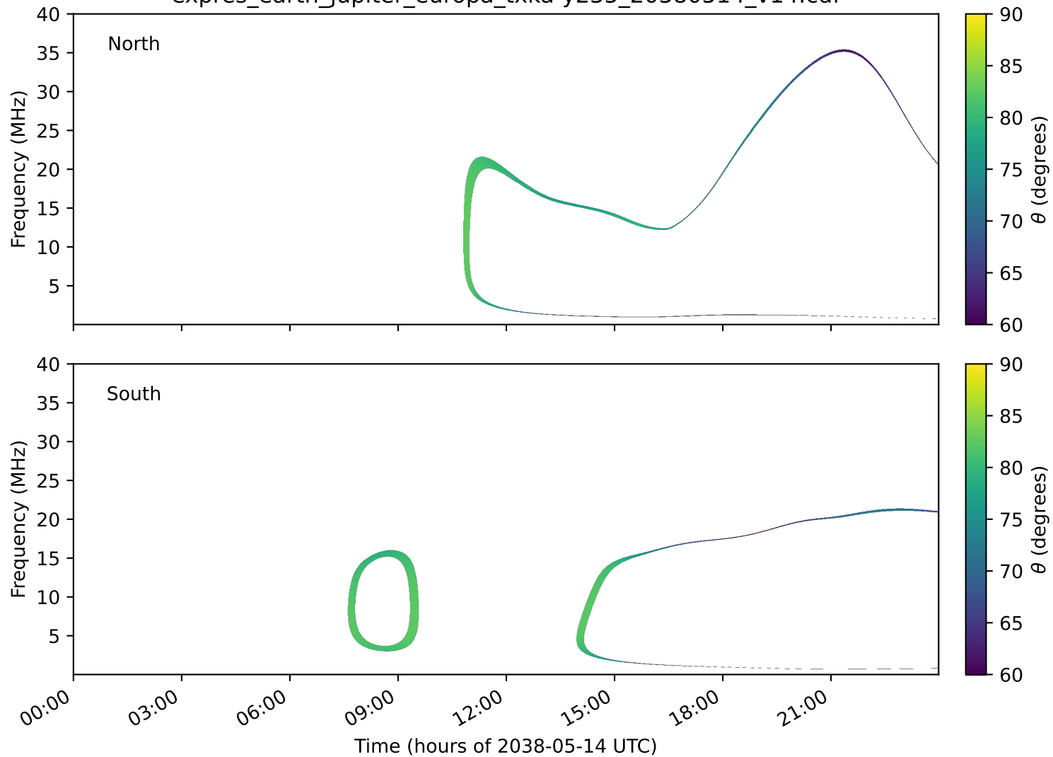
expres_earth_jupiter_europa_txka-y235_20380514_v14.cdf
