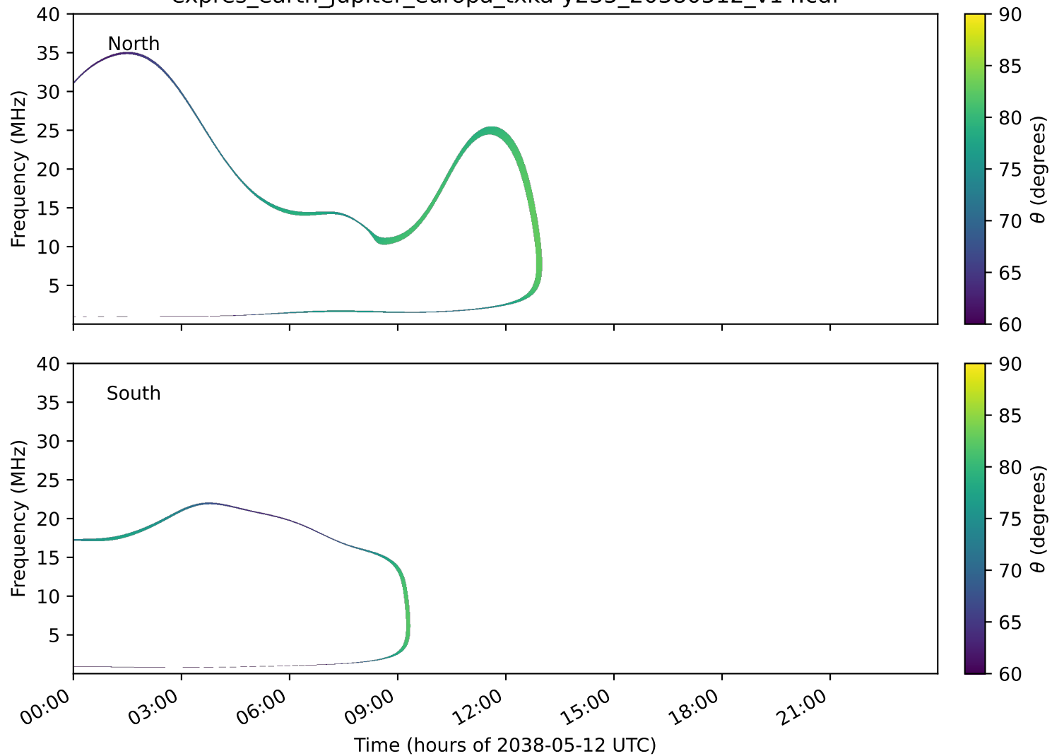
expres_earth_jupiter_europa_txka-y235_20380512_v14.cdf
