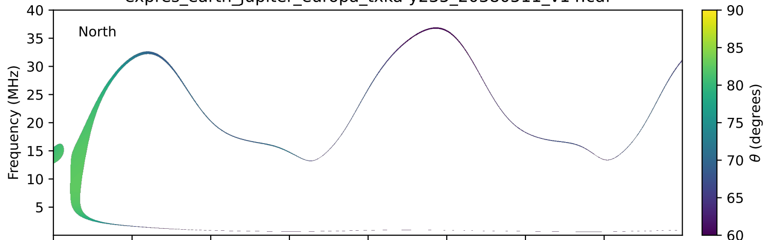
expres_earth_jupiter_europa_txka-y235_20380511_v14.cdf
