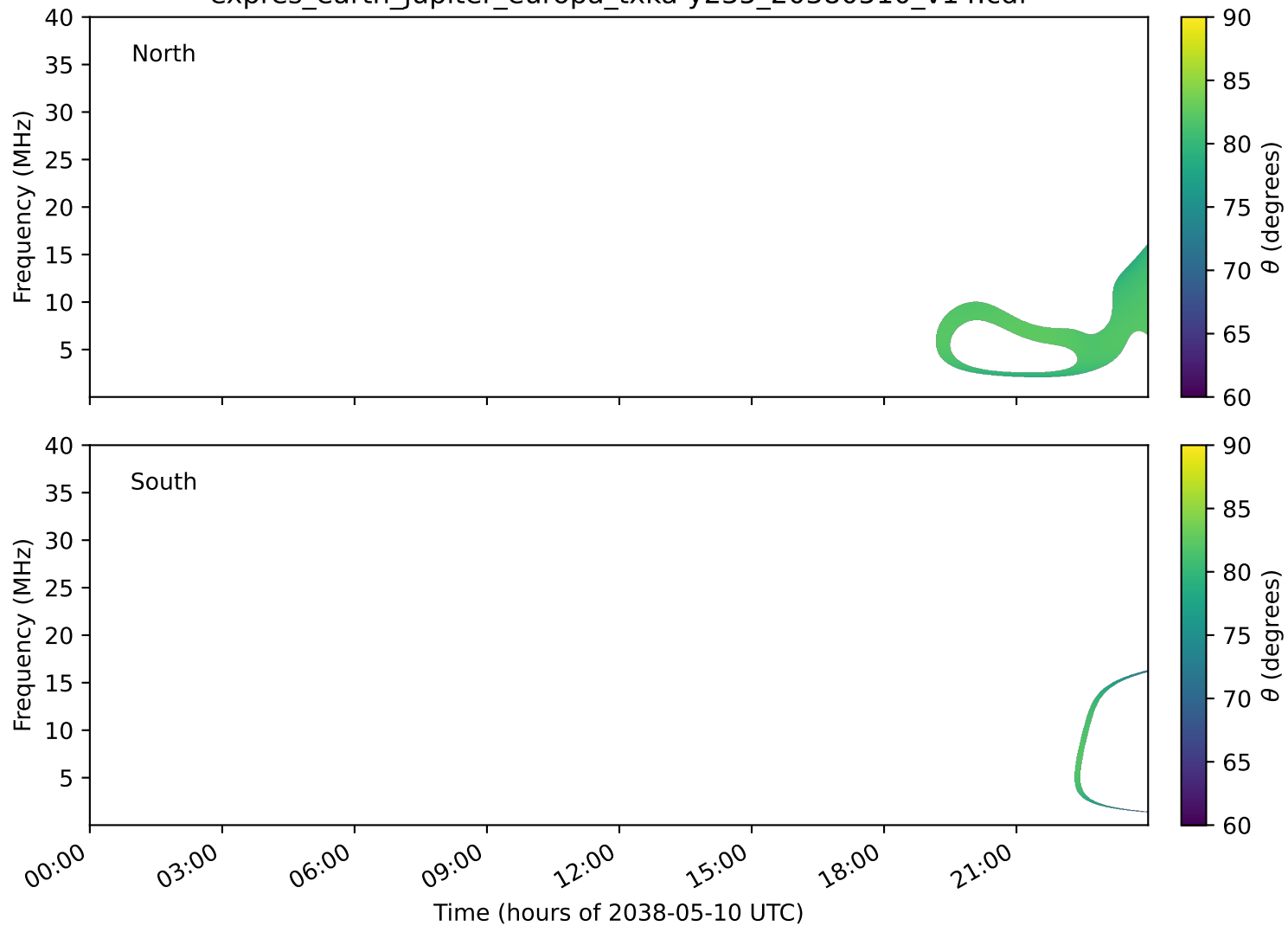
expres_earth_jupiter_europa_txka-y235_20380510_v14.cdf
