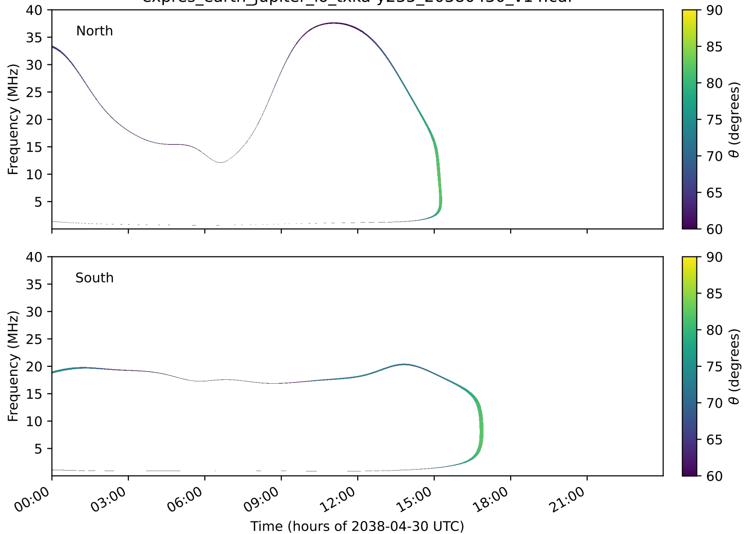
expres_earth_jupiter_io_txka-y235_20380430_v14.cdf
