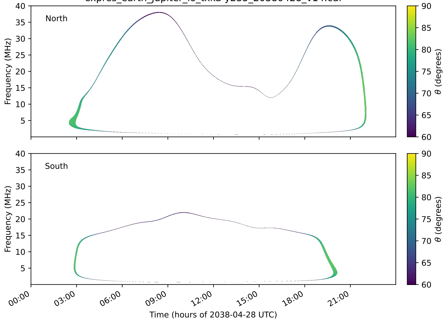
expres_earth_jupiter_io_txka-y235_20380428_v14.cdf
