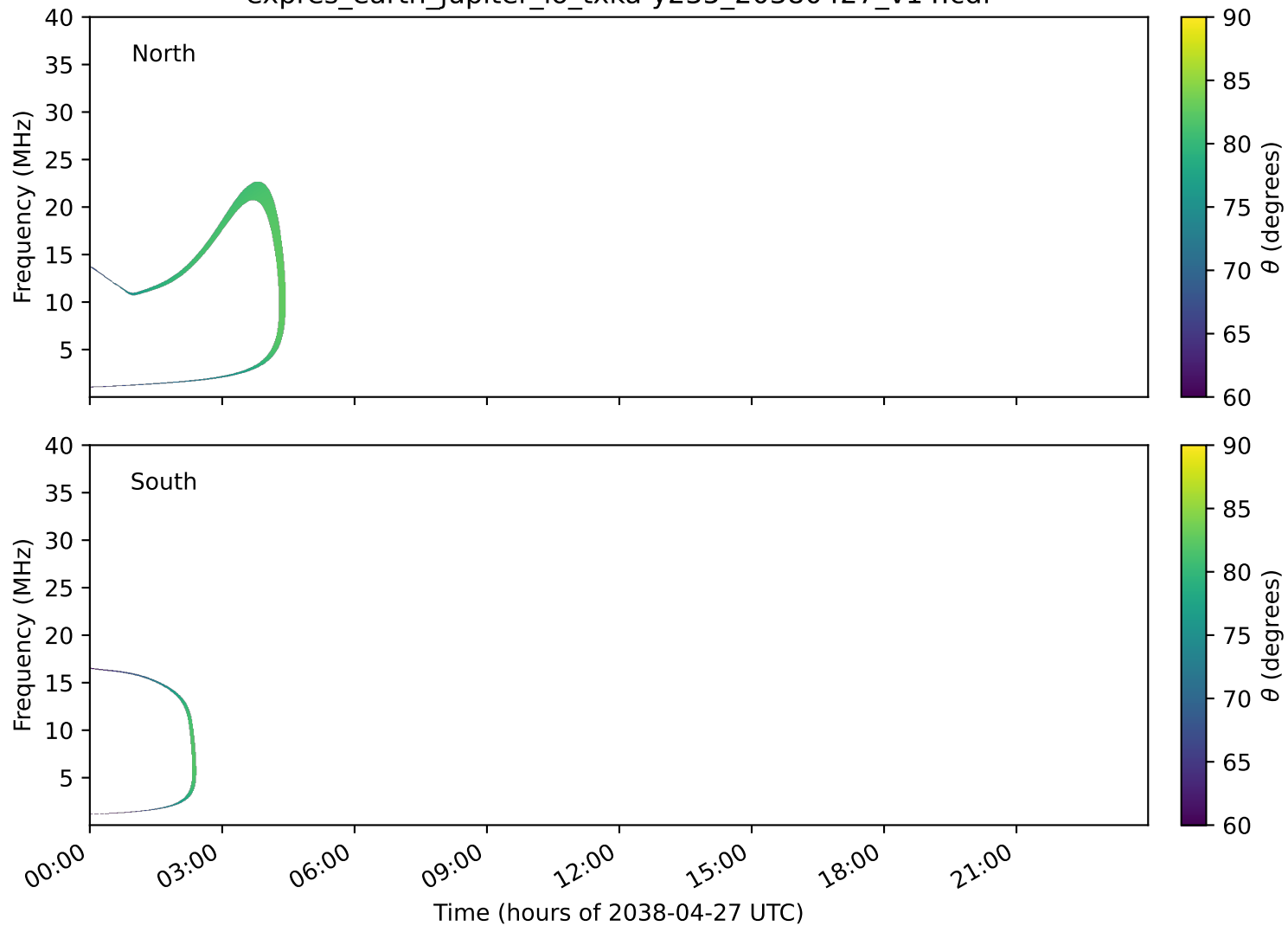
expres_earth_jupiter_io_txka-y235_20380427_v14.cdf
