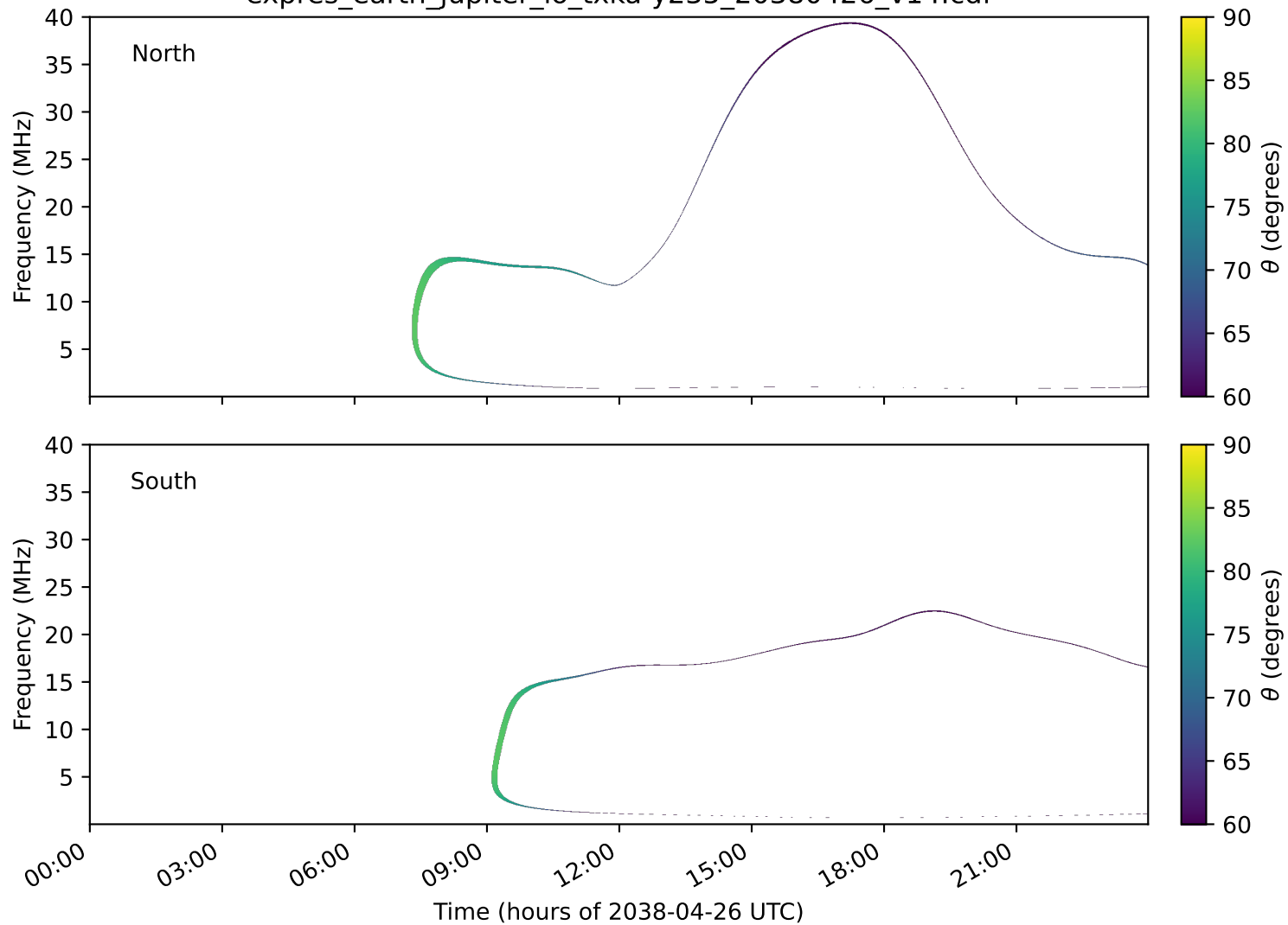
expres_earth_jupiter_io_txka-y235_20380426_v14.cdf
