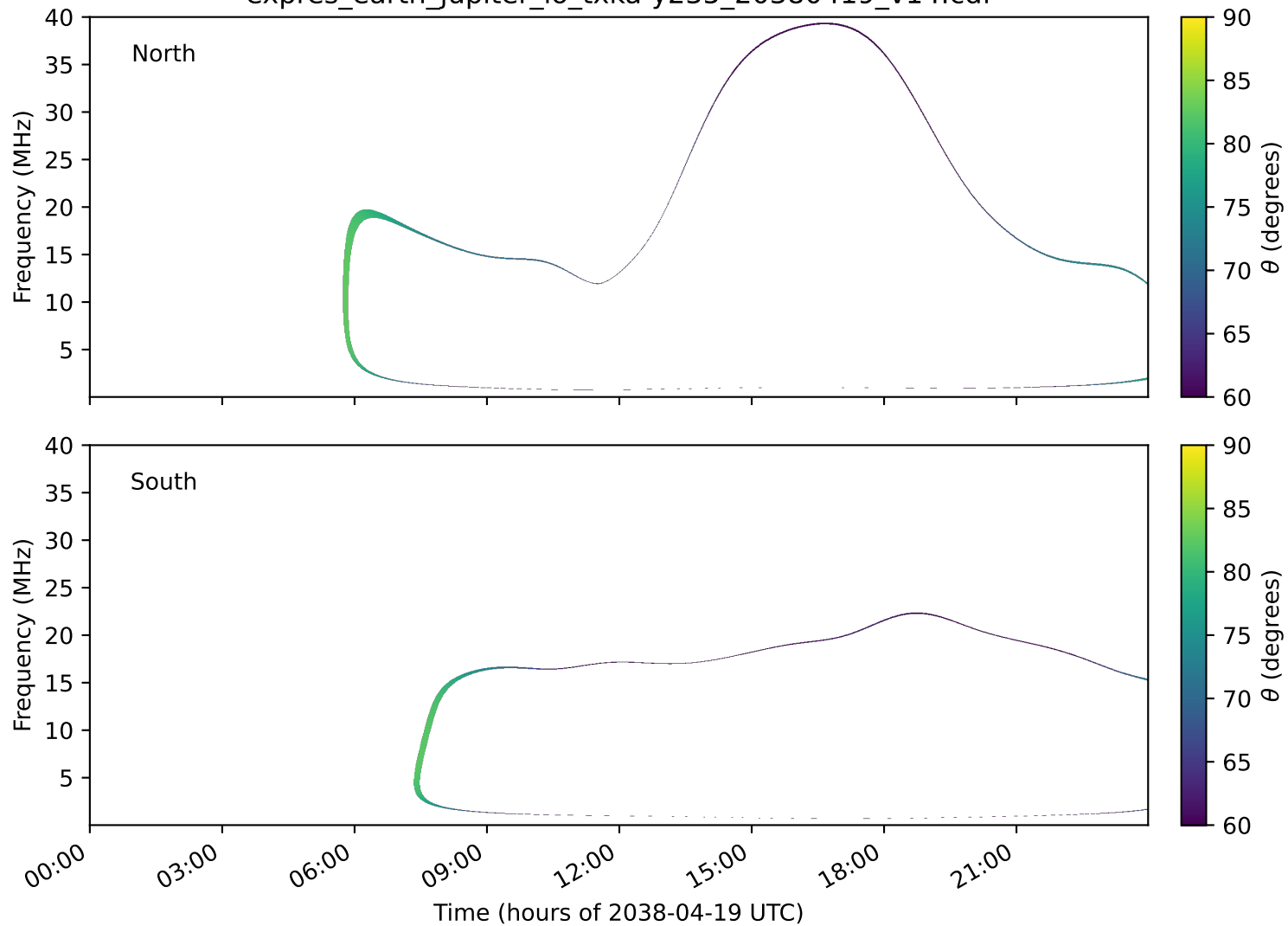
expres_earth_jupiter_io_txka-y235_20380419_v14.cdf
