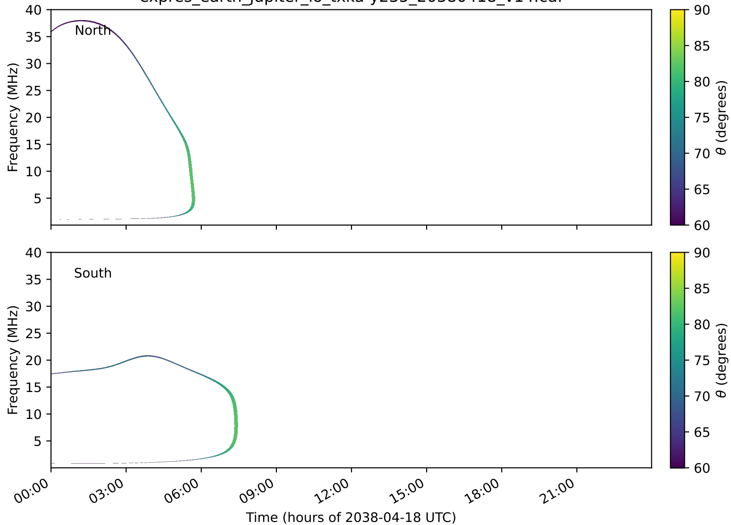
expres_earth_jupiter_io_txka-y235_20380418_v14.cdf
