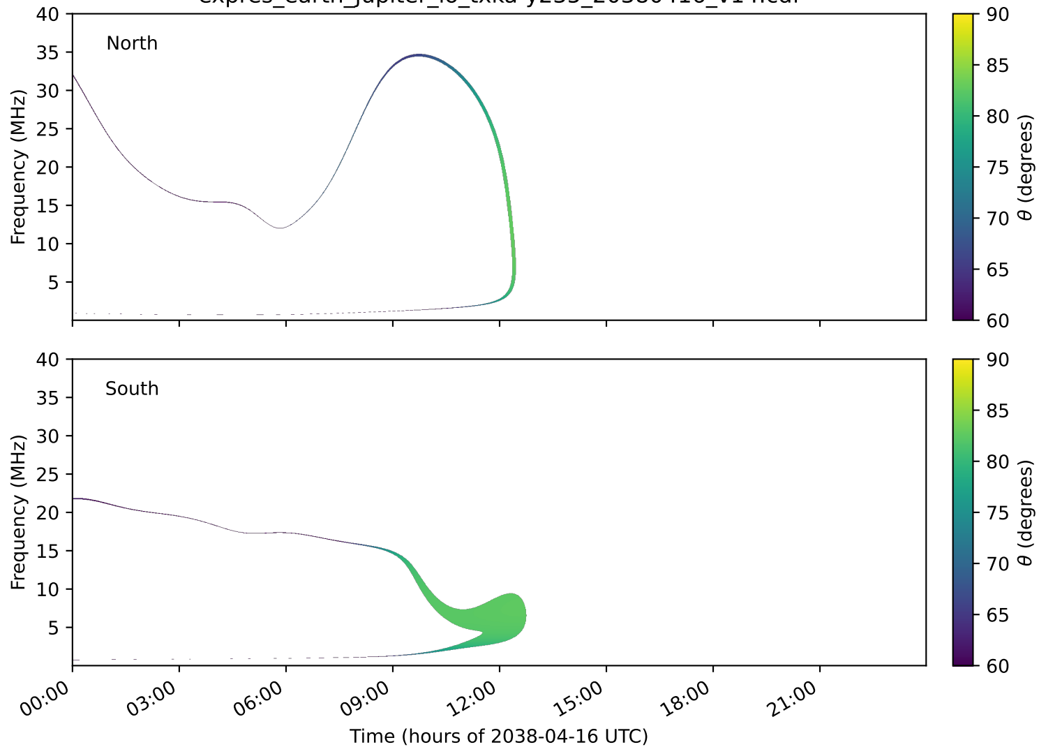
expres_earth_jupiter_io_txka-y235_20380416_v14.cdf
