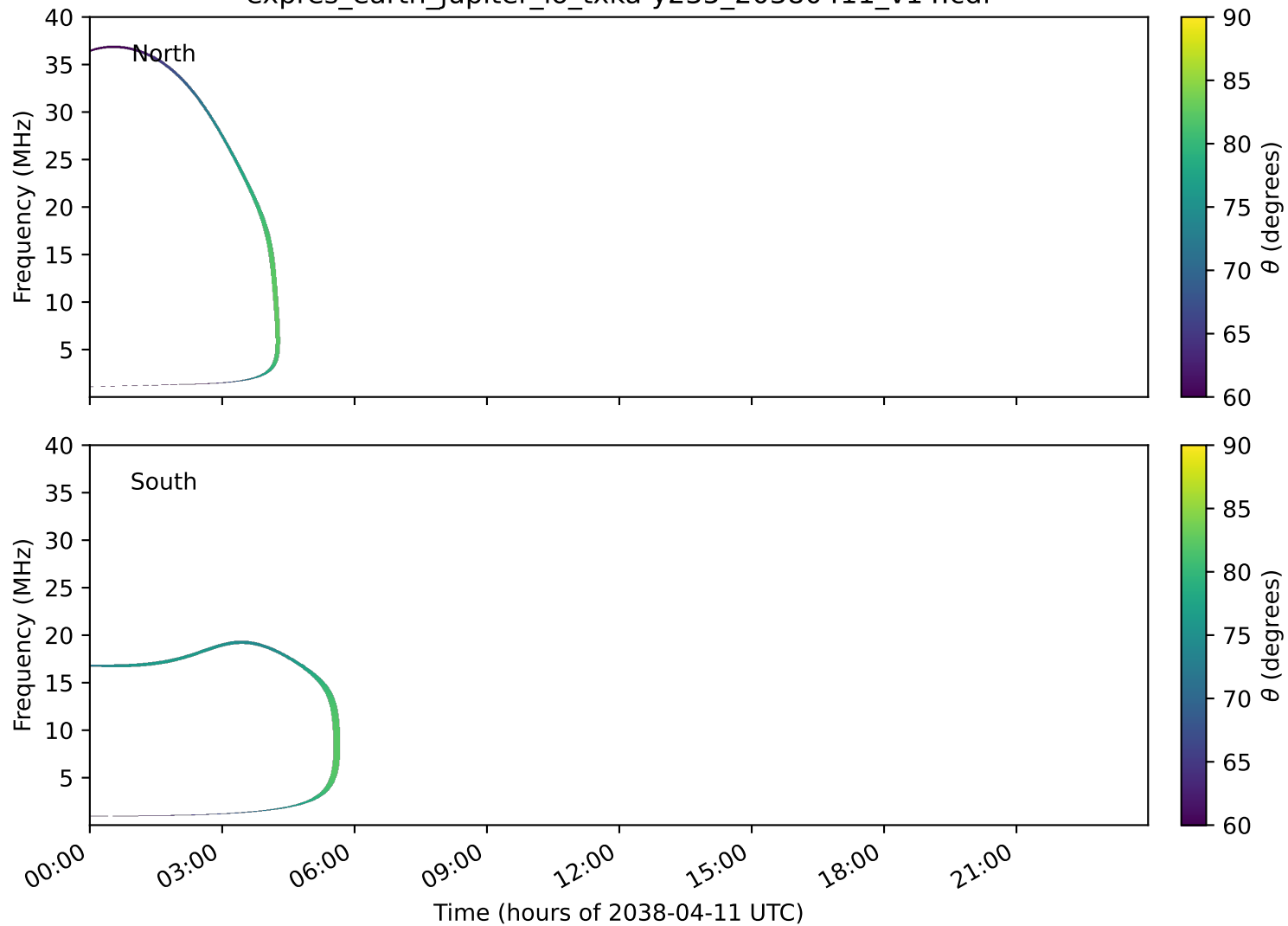
expres_earth_jupiter_io_txka-y235_20380411_v14.cdf
