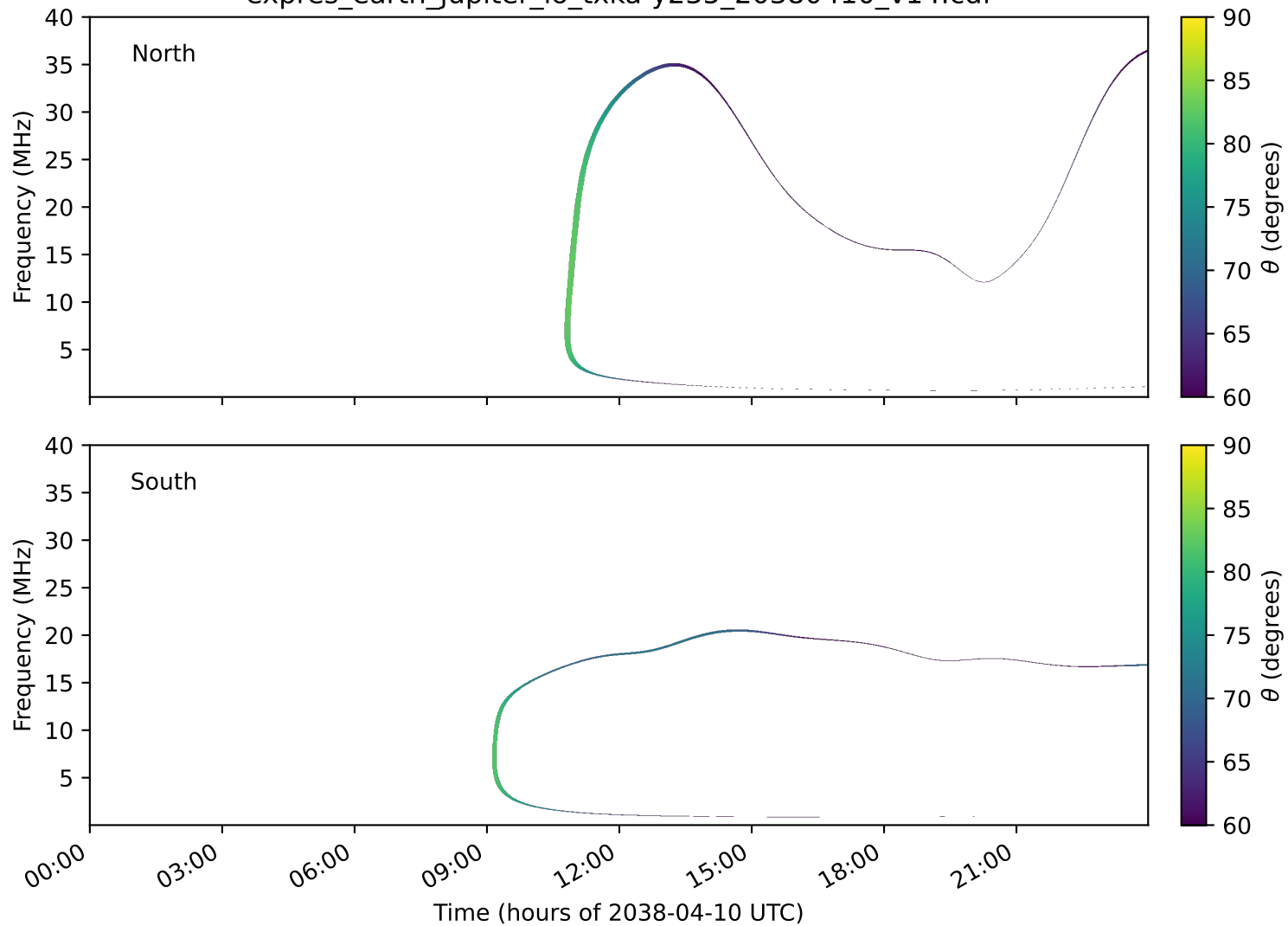
expres_earth_jupiter_io_txka-y235_20380410_v14.cdf
