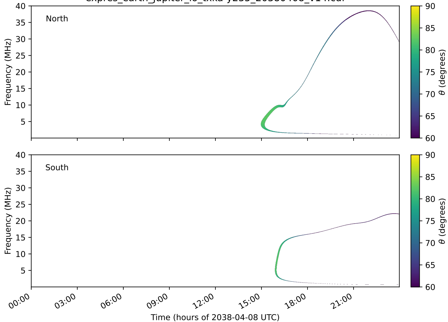
expres_earth_jupiter_io_txka-y235_20380408_v14.cdf
