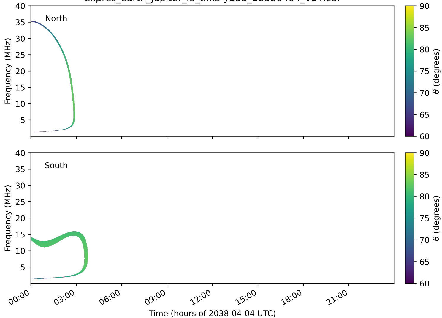
expres_earth_jupiter_io_txka-y235_20380404_v14.cdf
