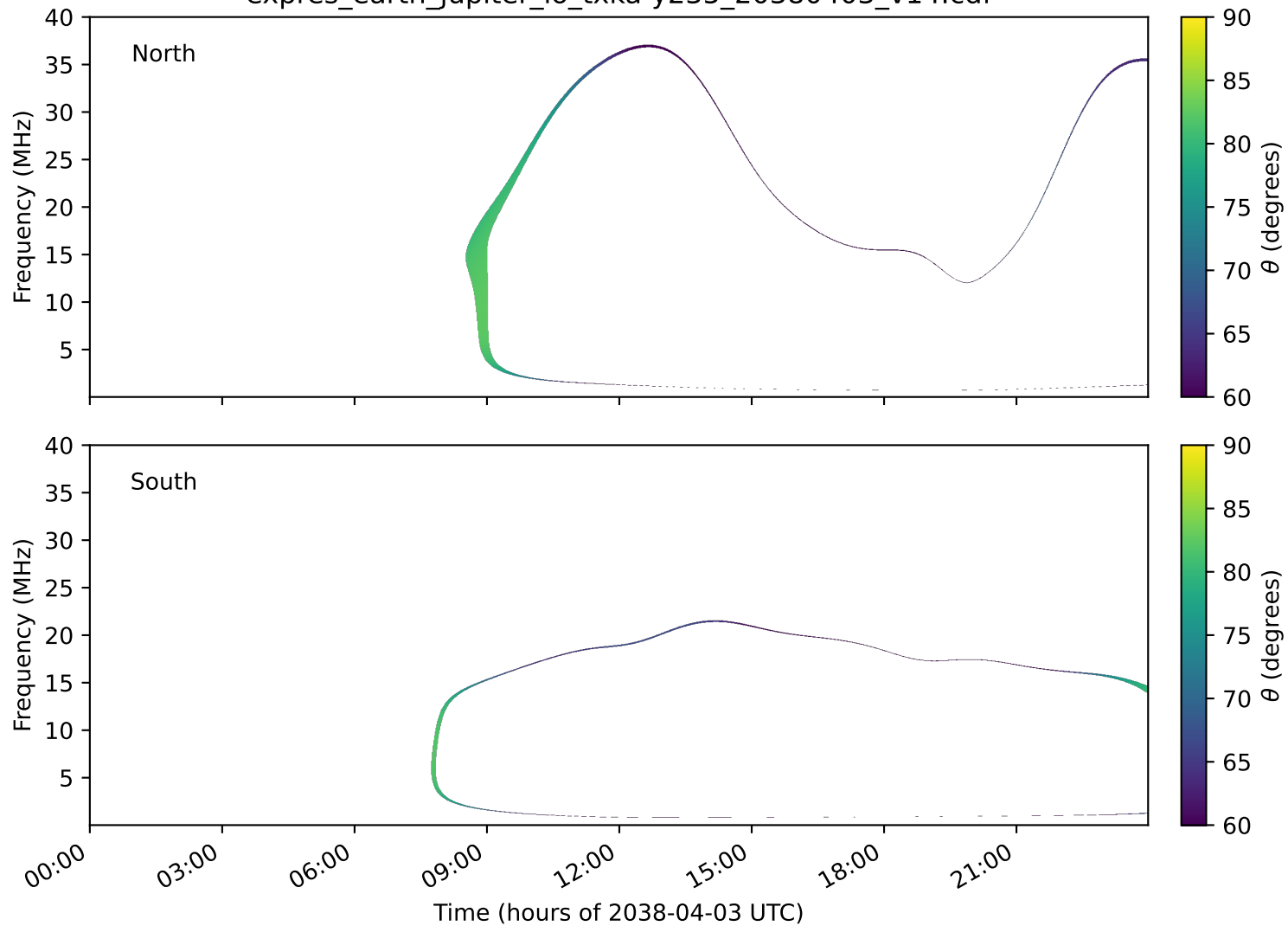
expres_earth_jupiter_io_txka-y235_20380403_v14.cdf
