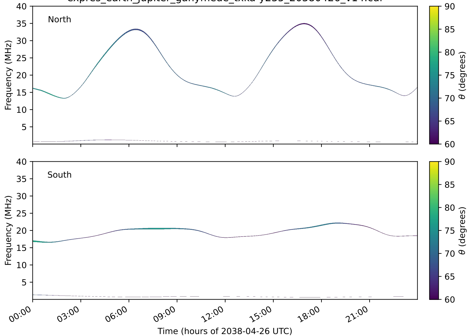
expres_earth_jupiter_ganymede_txka-y235_20380426_v14.cdf
