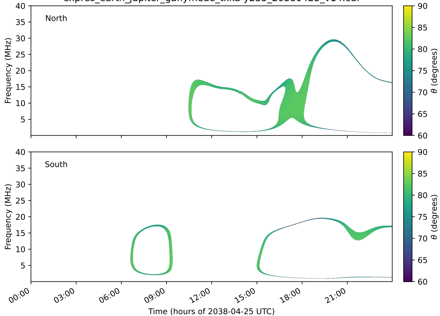
expres_earth_jupiter_ganymede_txka-y235_20380425_v14.cdf
