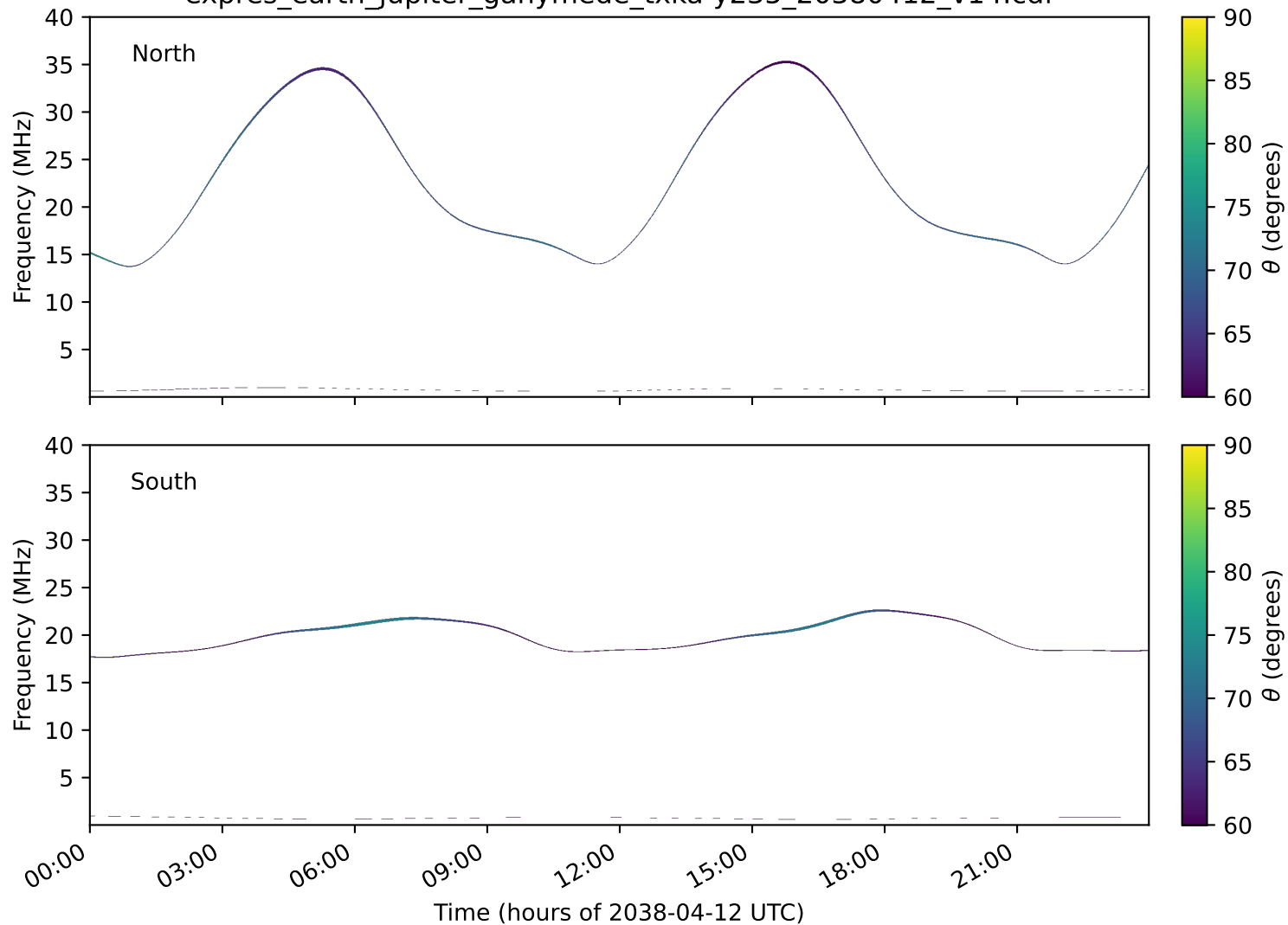
expres_earth_jupiter_ganymede_txka-y235_20380412_v14.cdf
