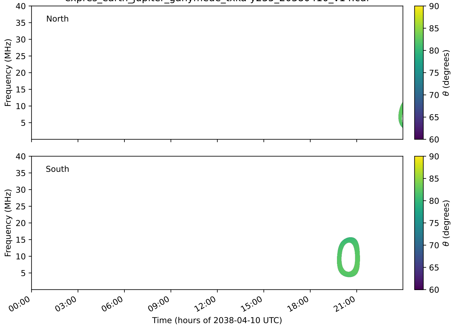
expres_earth_jupiter_ganymede_txka-y235_20380410_v14.cdf
