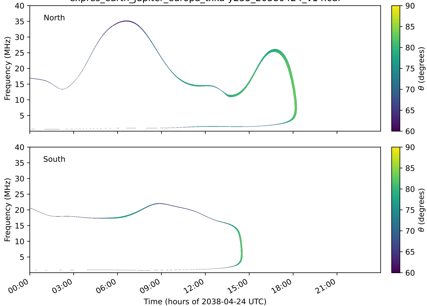
expres_earth_jupiter_europa_txka-y235_20380424_v14.cdf
