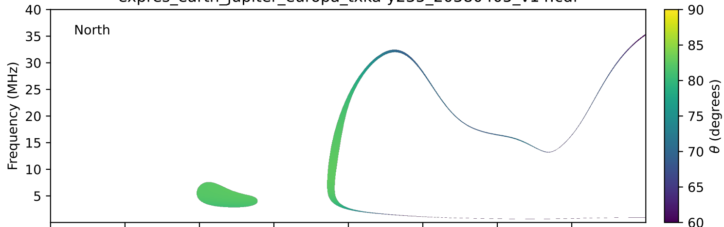
expres_earth_jupiter_europa_txka-y235_20380405_v14.cdf
