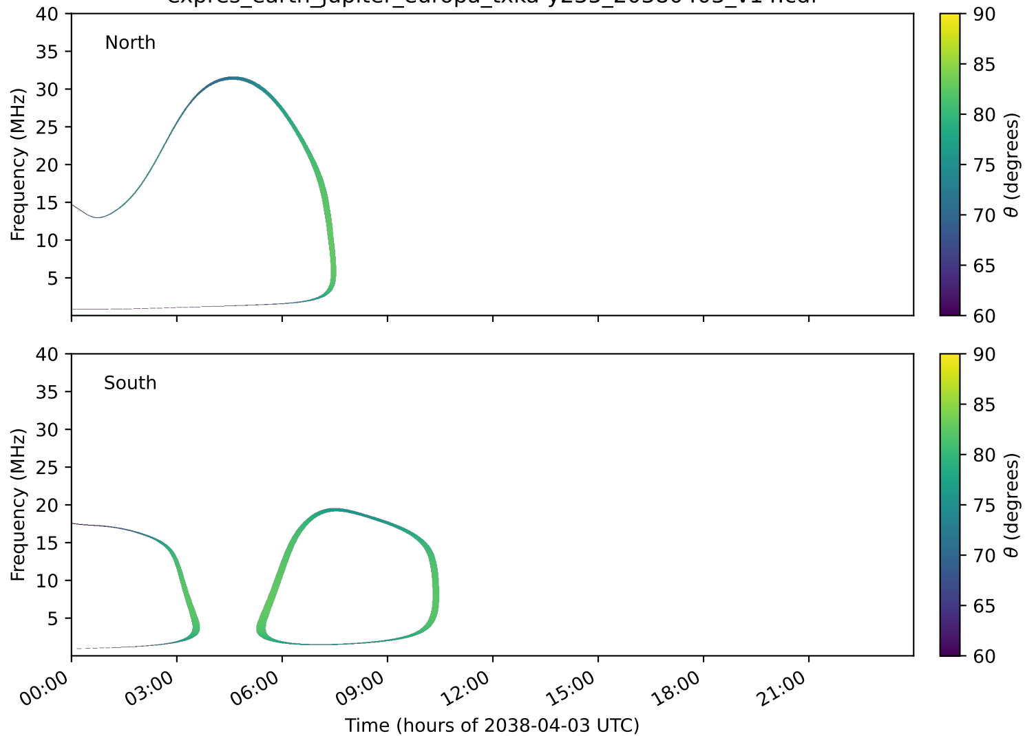
expres_earth_jupiter_europa_txka-y235_20380403_v14.cdf
