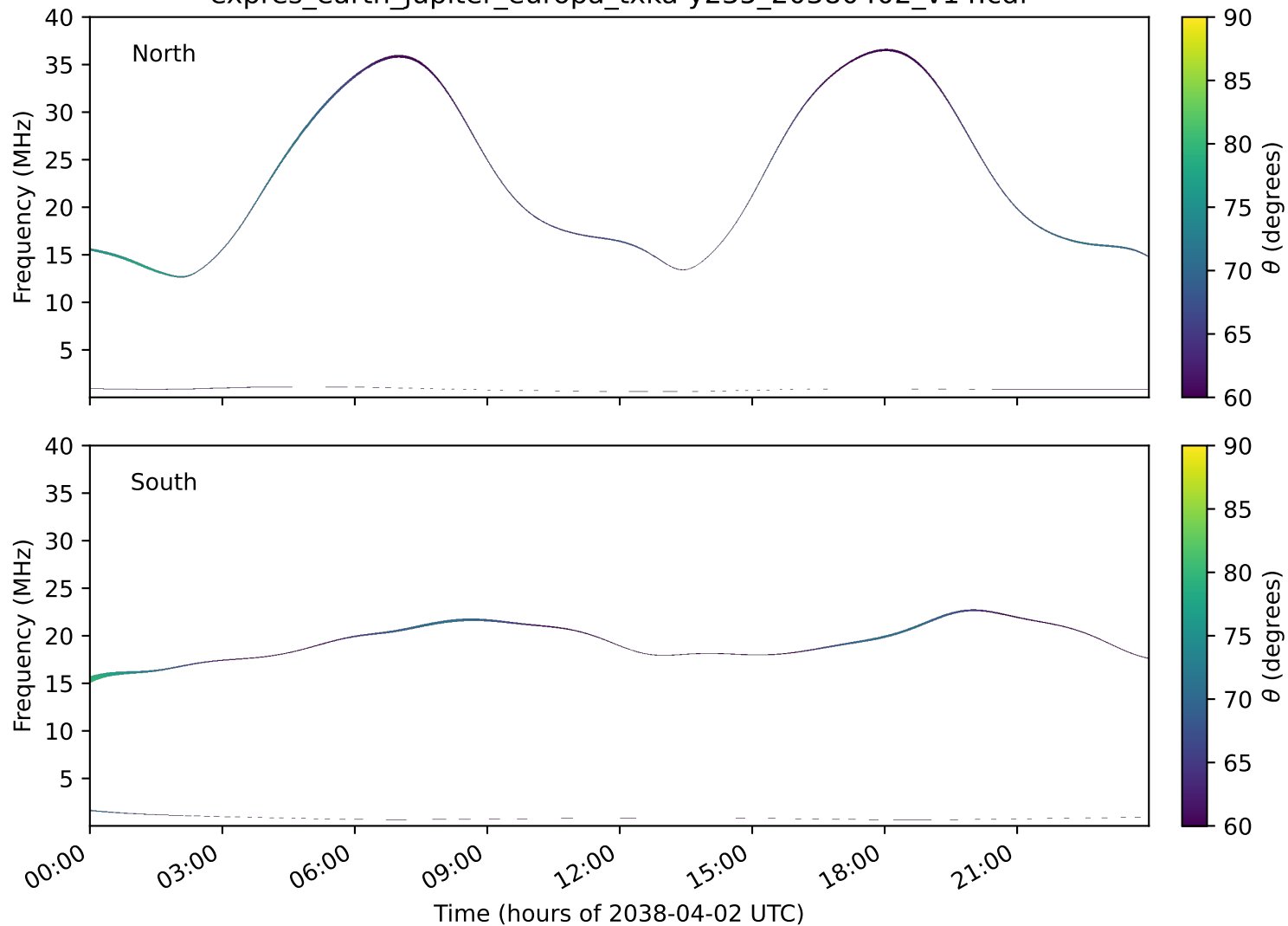
expres_earth_jupiter_europa_txka-y235_20380402_v14.cdf
