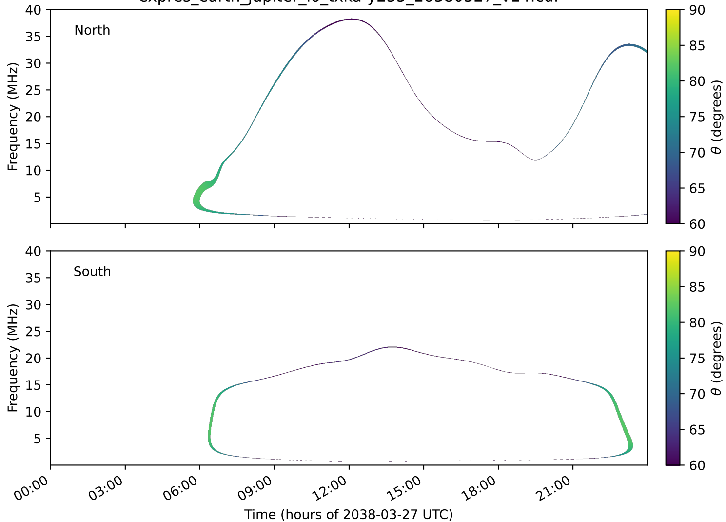
expres_earth_jupiter_io_txka-y235_20380327_v14.cdf
