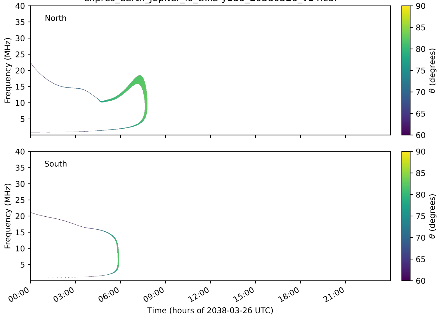
expres_earth_jupiter_io_txka-y235_20380326_v14.cdf
